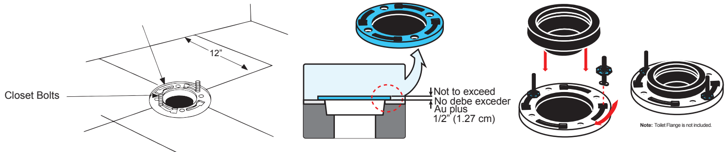
Closet Flange
